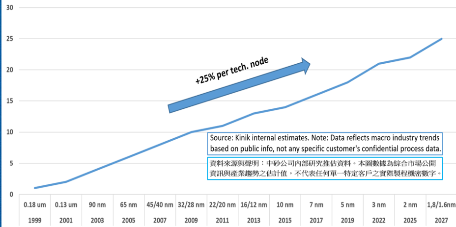
Logic IC CMP layer No. vs. Tech. Nodes (excludes adv. packaging)
